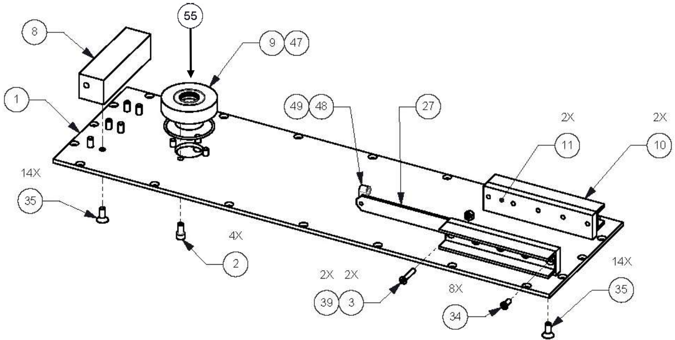
TOP PLATE COMPONENTS
