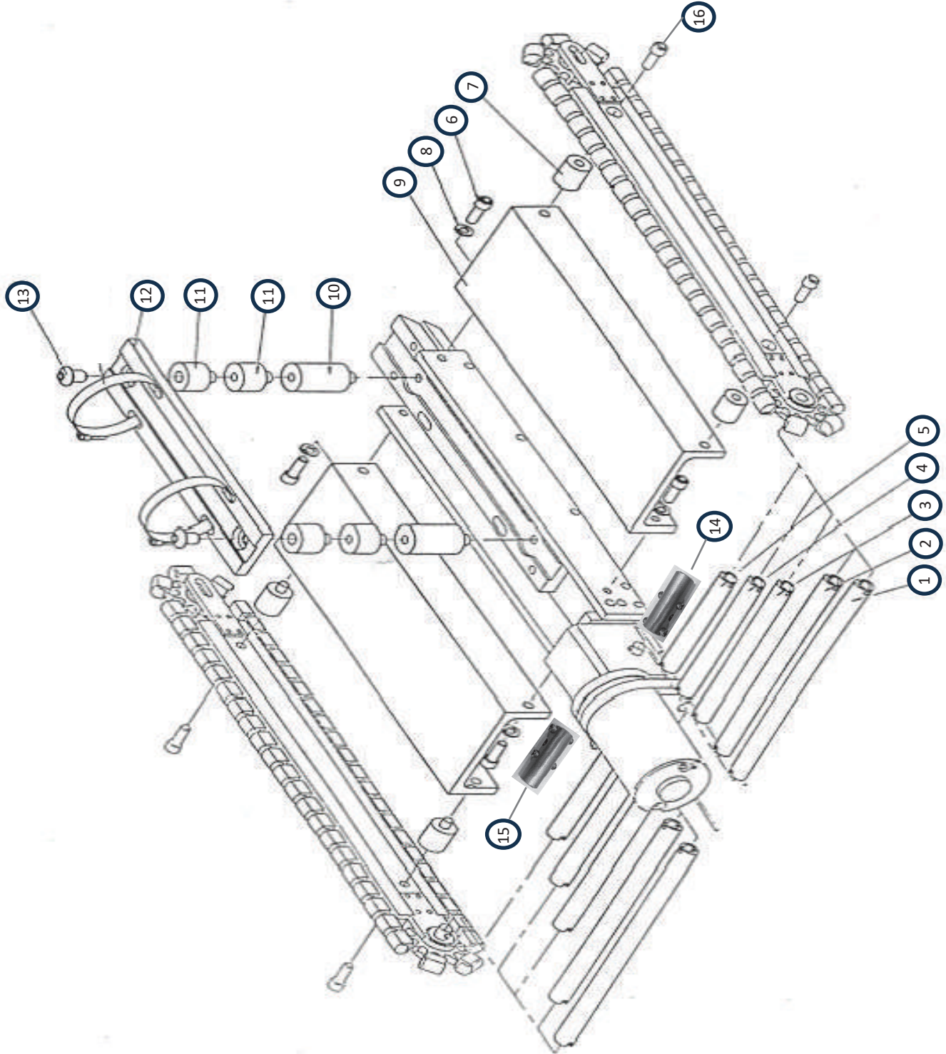
PROTRAK 18"-30" EXTENSION ILLUSTRATION 840-37276
